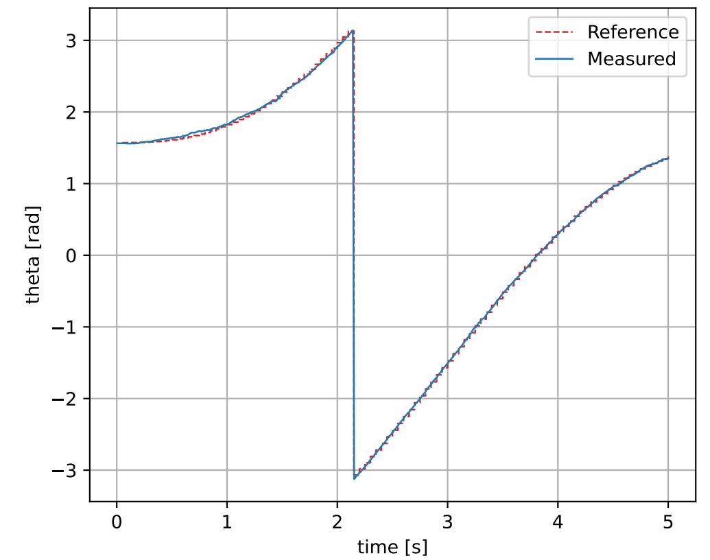
theta State
