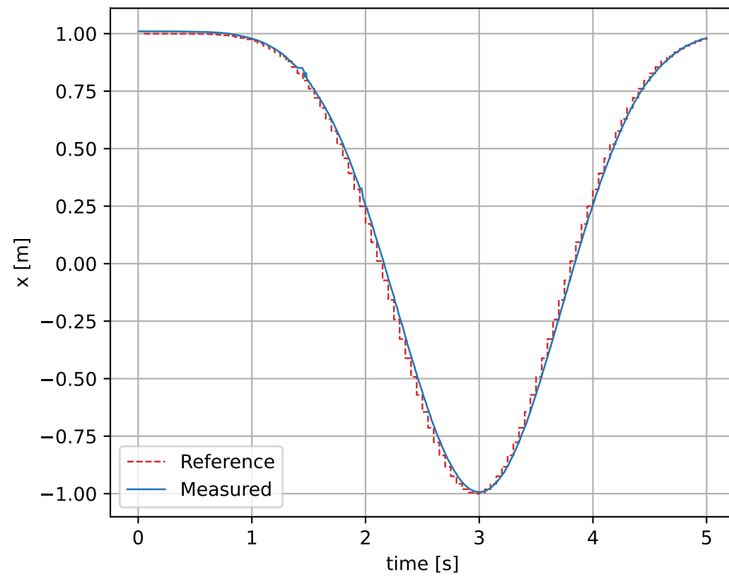
x State
